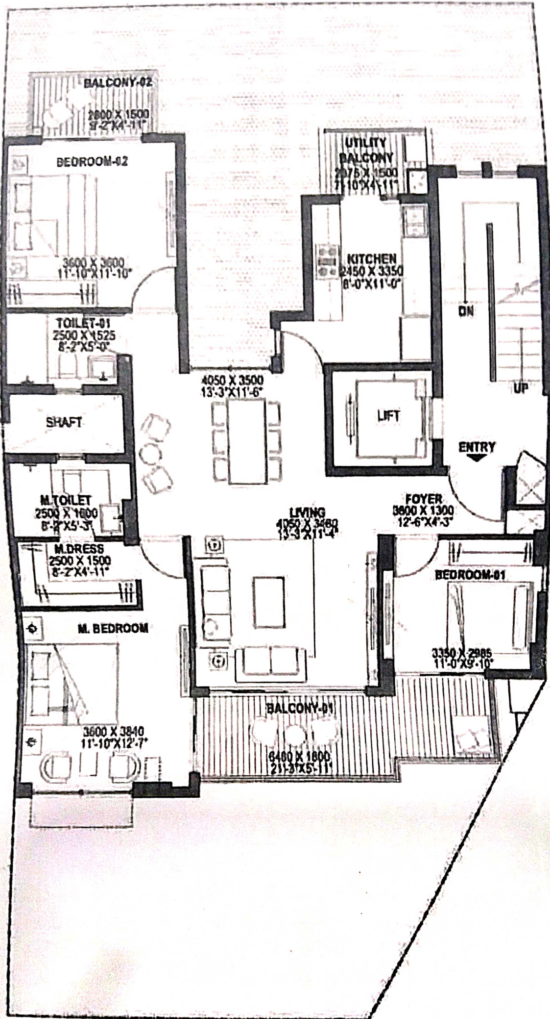
TYPICAL FLOOR PLAN 1234
